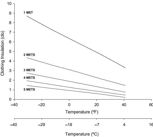
FIGURE 2 —Approximate amount of clothing insulation needed at different air temperatures and physical activity levels. Wind speed is assumed to be less than 5 mph (2.2 m·s -1 ). One MET refers to energy expenditure at rest. One clo of insulation is the clothing necessary to allow a resting person to be comfortable when the air temperature is 21°C (70°F) (7). Refer to Table 4 for a list of typical clothing ensembles and their respective clo values.
